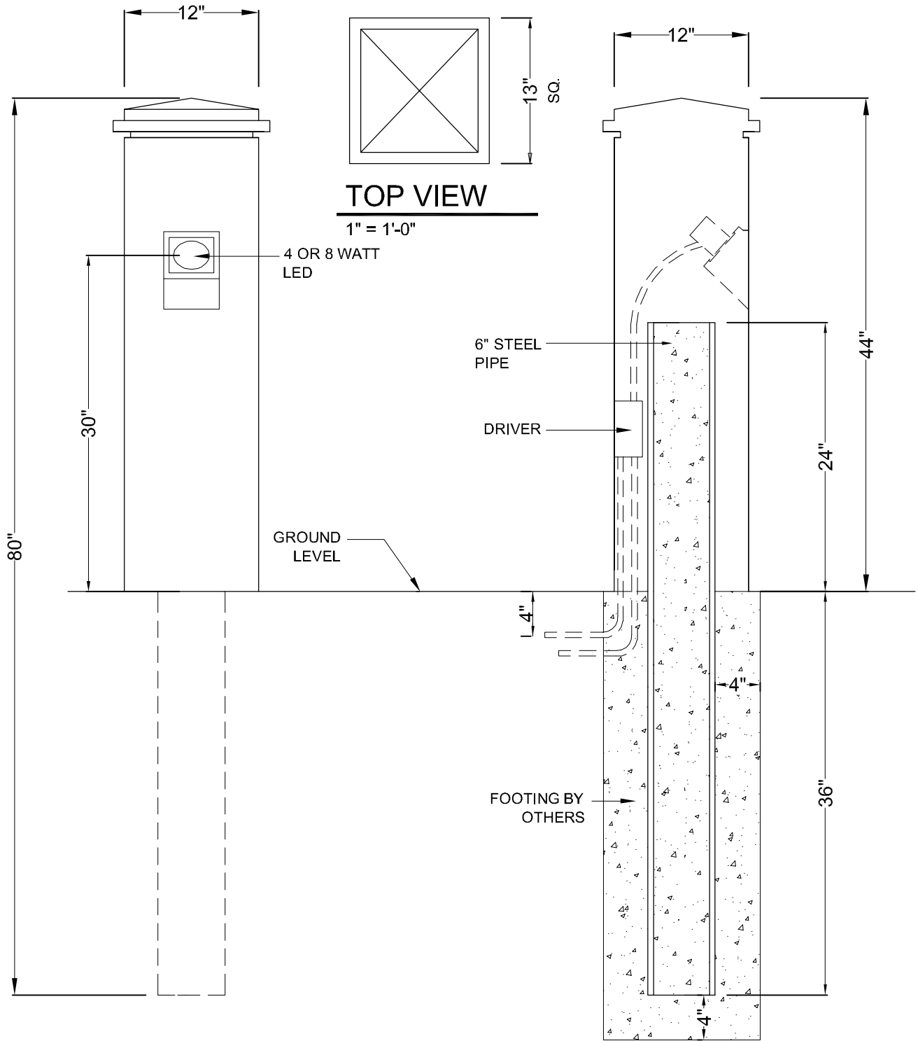
1 FRONT ELEVATION 1" = 1'-0"
