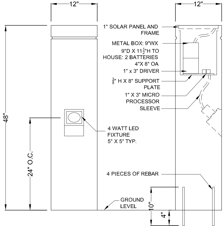
2 FRONT ELEVATION 1" = 1'-0"
